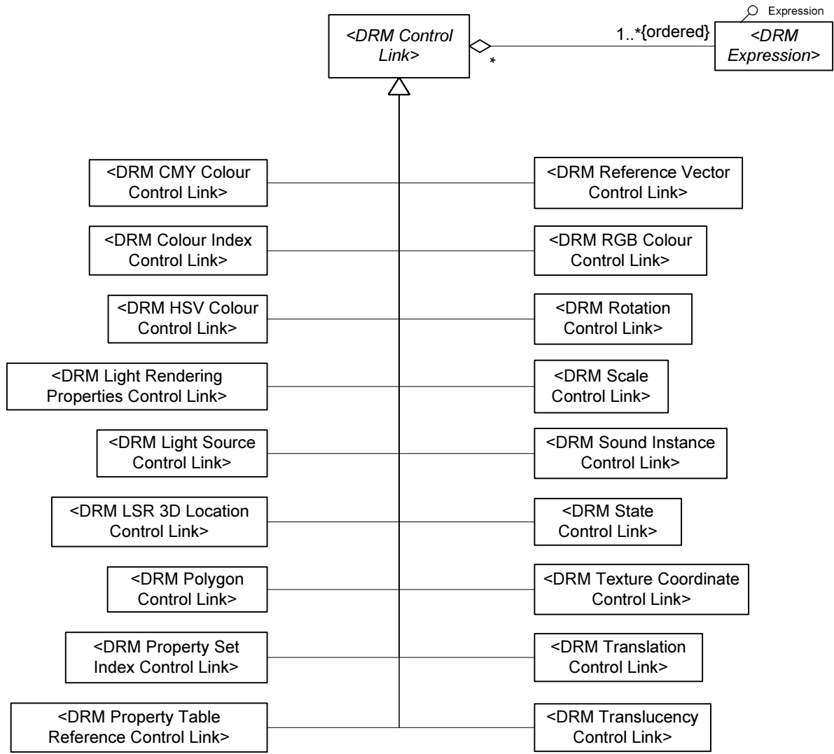
Sheet 17 — Control link (Version 4.1)
