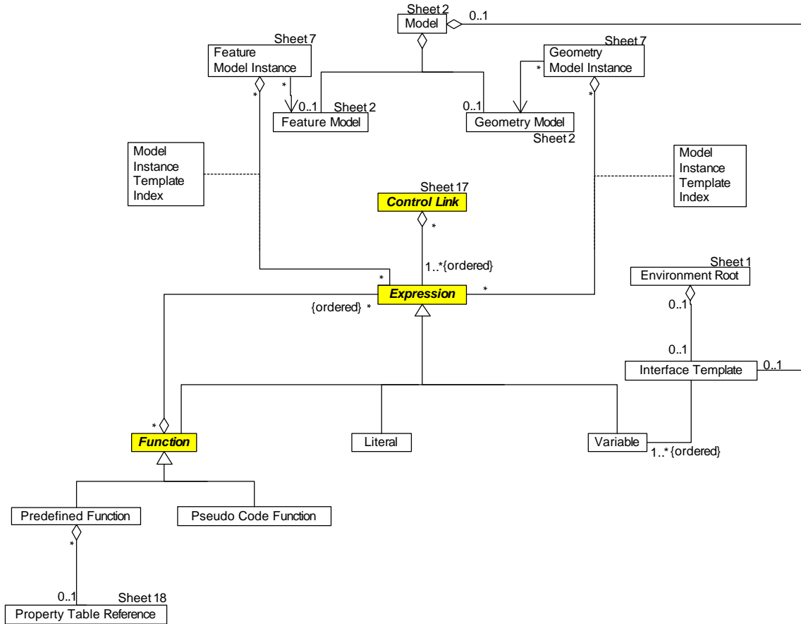
Diagram A.16: Expressions
