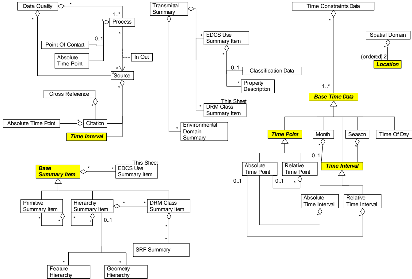
Diagram A.20: Time and Metadata
