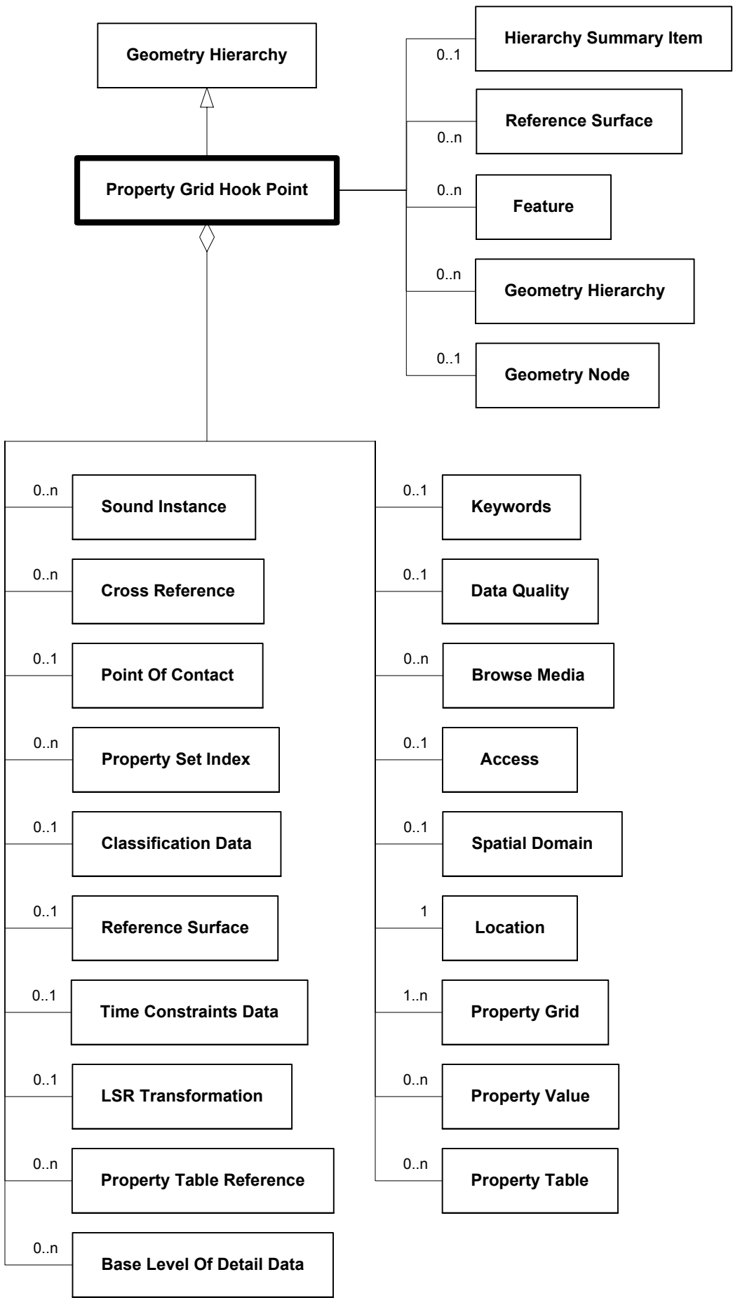
Figure 6.223—DRM_Property_Grid_Hook_Point
