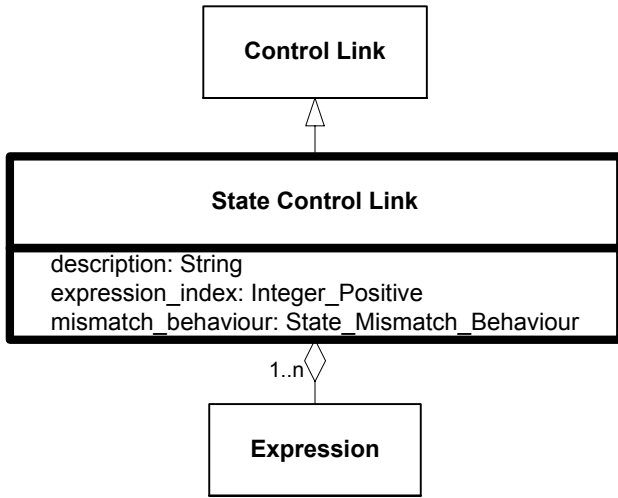
Figure 6.304—DRM_State_Control_Link
