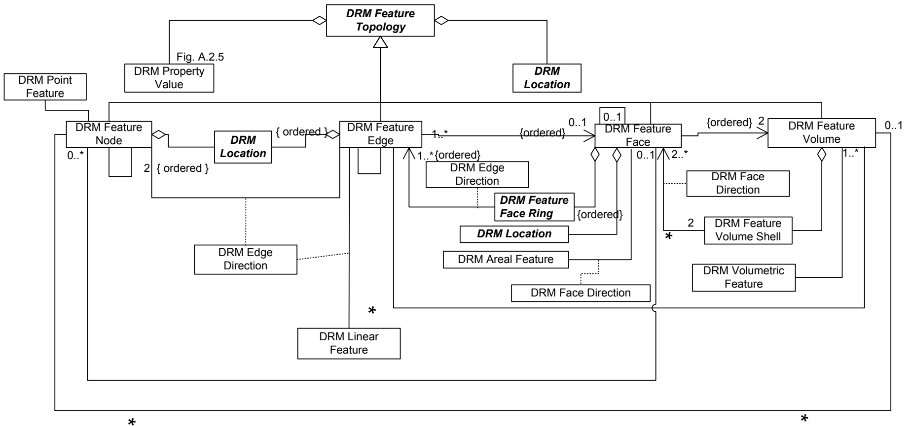
Figure A.2.12 DRM Feature Topology
