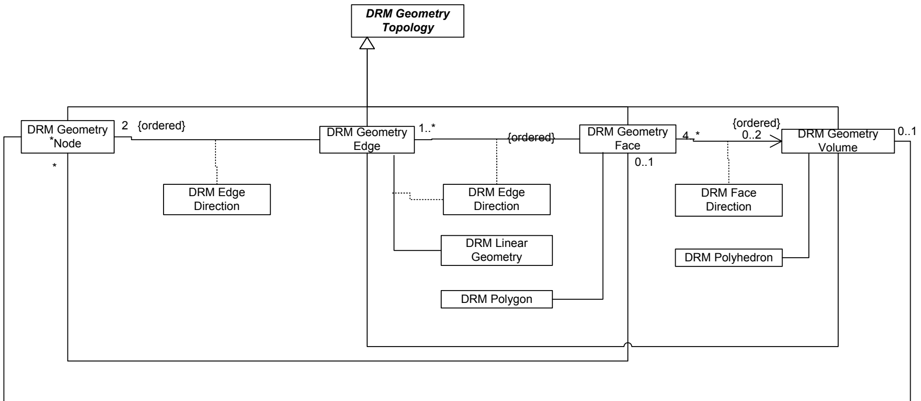
Figure A.2.13 DRM Geometry Topology
