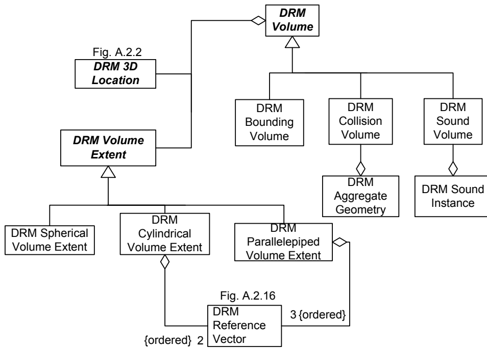
Figure A.2.3 Base Data Classes, DRM Reference Surface, and DRM Volume
