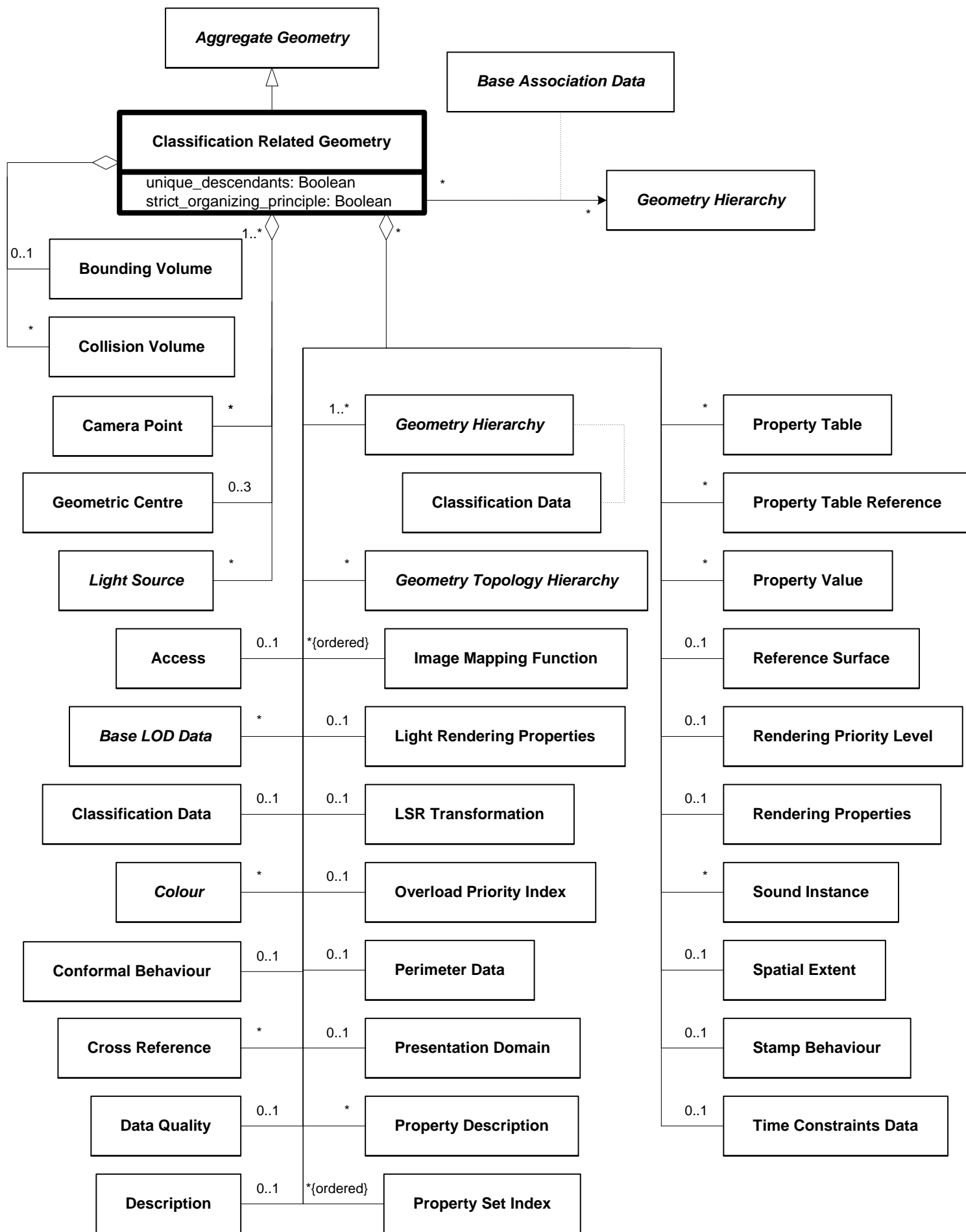
Figure 6.34 — DRM_Classification_Related_Geometry
