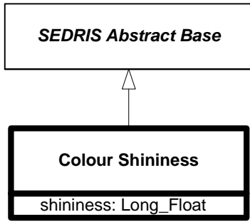
Figure 6.45 — DRM_Colour_Shininess
