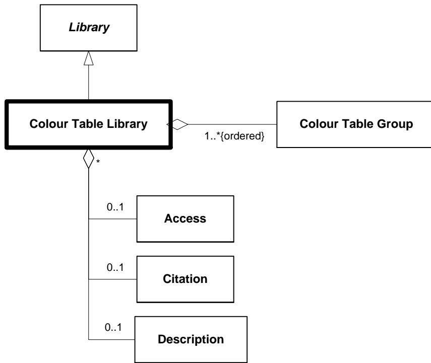
Figure 6.48 — DRM_Colour_Table_Library
