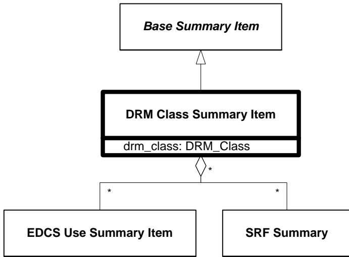
Figure 6.68 — DRM_DRM_Class_Summary_Item
