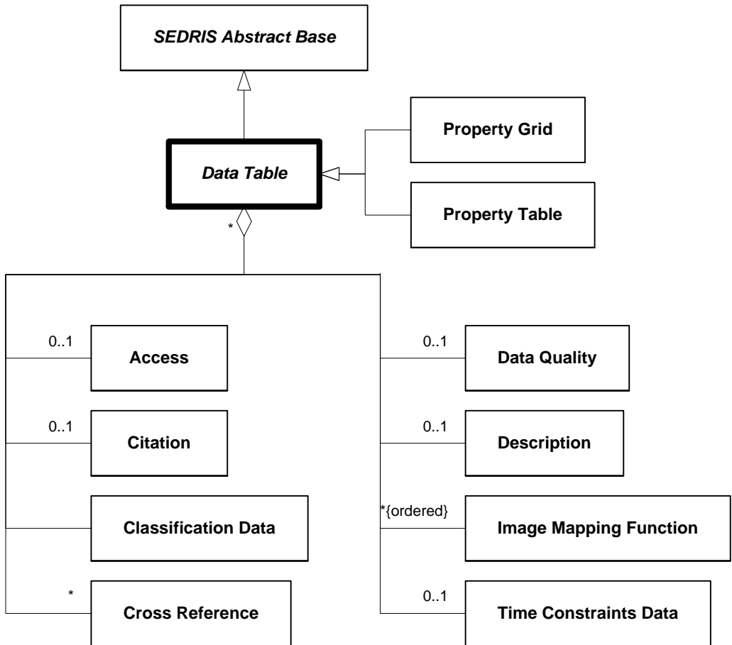
Figure 6.62 — DRM_Data_Table
