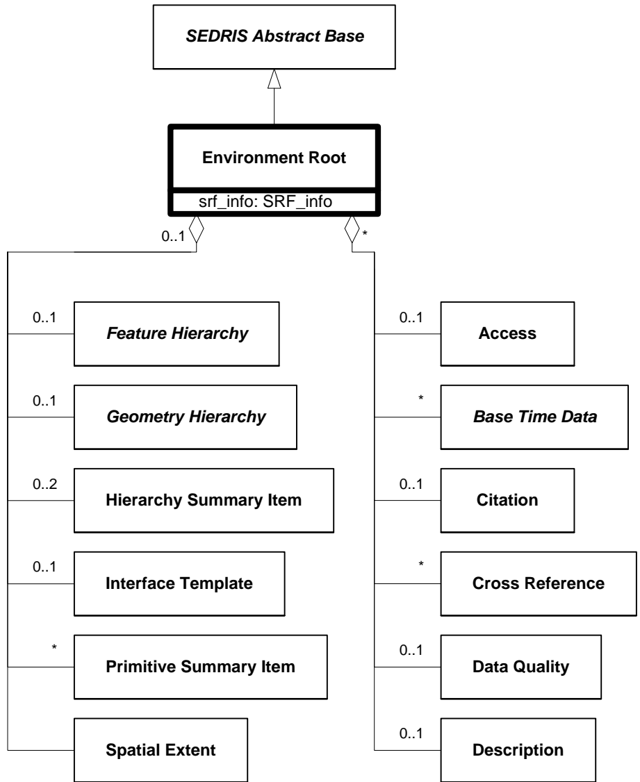
Figure 6.81 — DRM_Environment_Root
