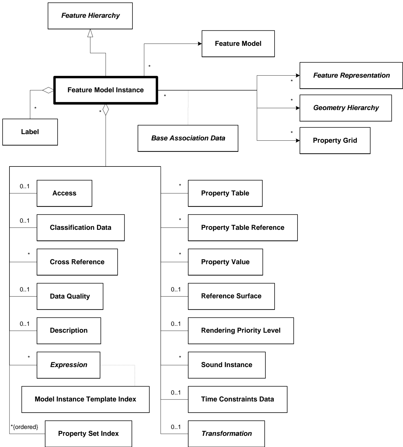
Figure 6.92 — DRM_Feature_Model_Instance
