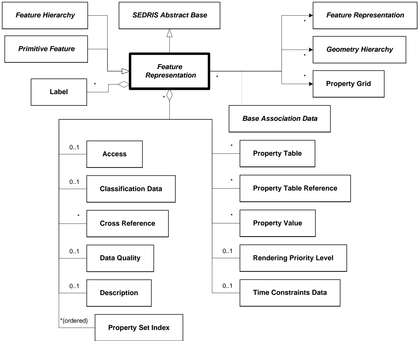
Figure 6.94 — DRM_Feature_Representation
