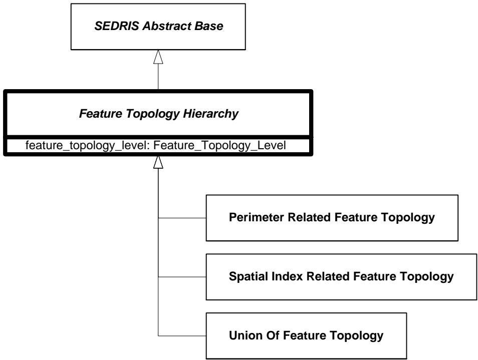
Figure 6.96 — DRM_Feature_Topology_Hierarchy
