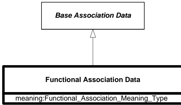
Figure 6.103 — DRM_Functional_Association_Data
