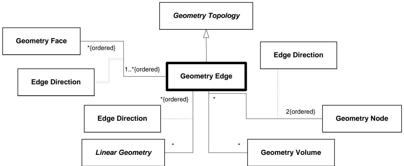
Figure 6.108 — DRM_Geometry_Edge
