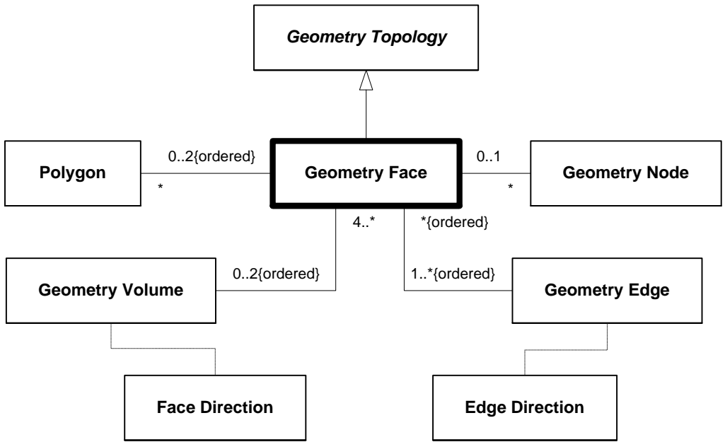
Figure 6.109 — DRM_Geometry_Face
