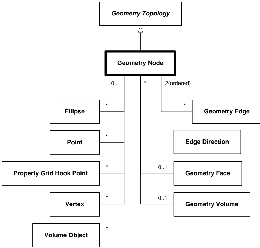
Figure 6.113 — DRM_Geometry_Node
