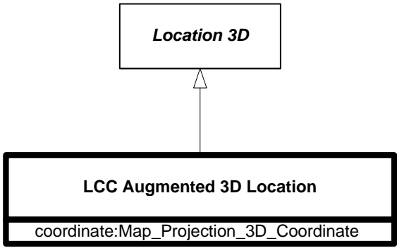
Figure 6.145 — DRM_LCC_Augmented_3D_Location
