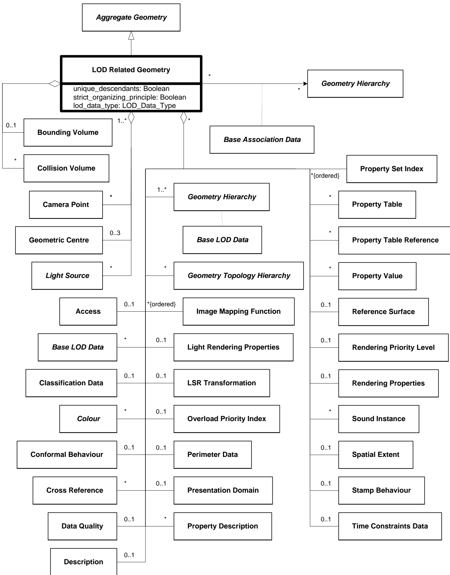
Figure 6.166 — DRM_LOD_Related_Geometry
