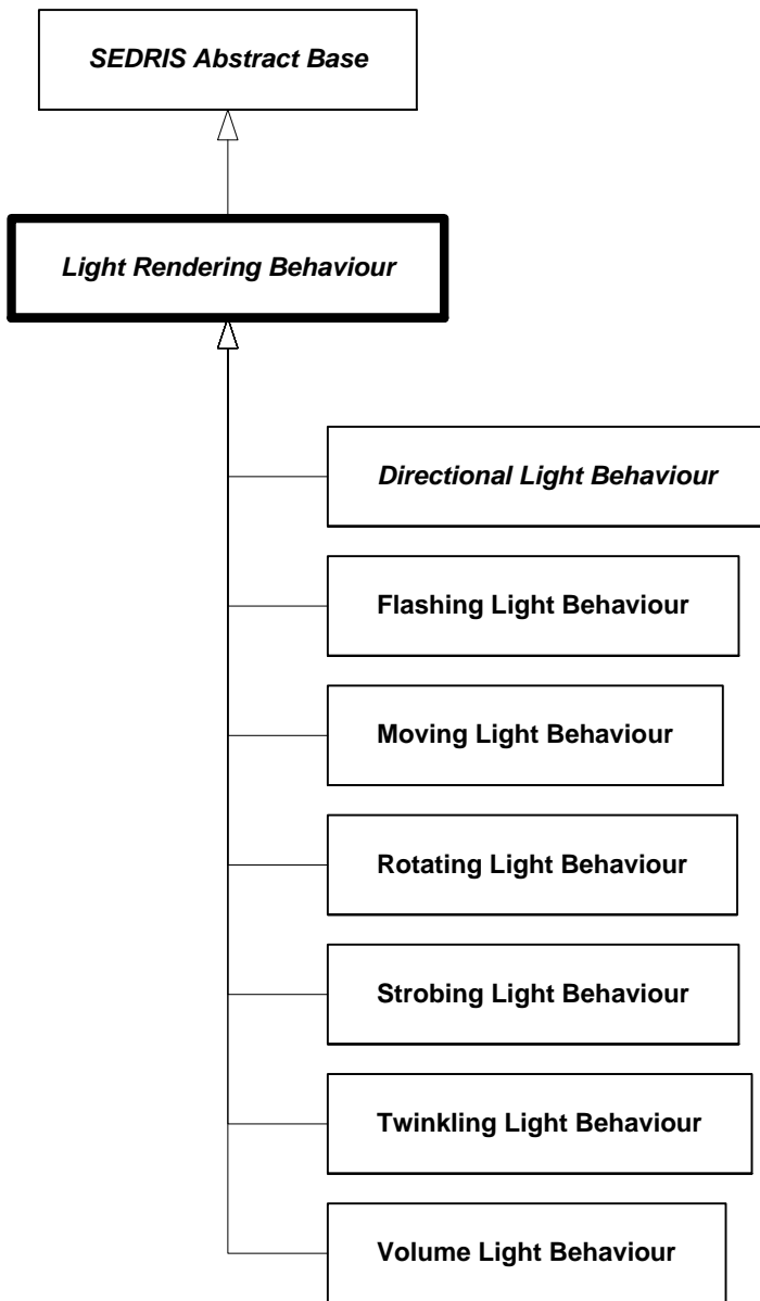
Figure 6.148 — DRM_Light_Rendering_Behaviour
