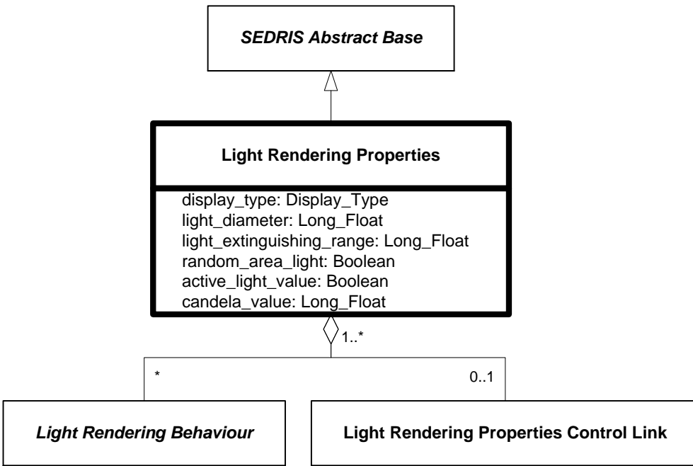
Figure 6.149 — DRM_Light_Rendering_Properties
