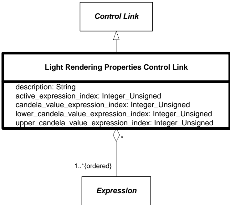
Figure 6.150 — DRM_Light_Rendering_Properties_Control_Link
