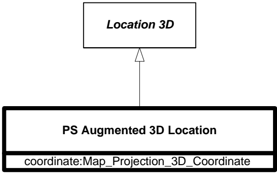
Figure 6.243 — DRM_PS_Augmented_3D_Location
