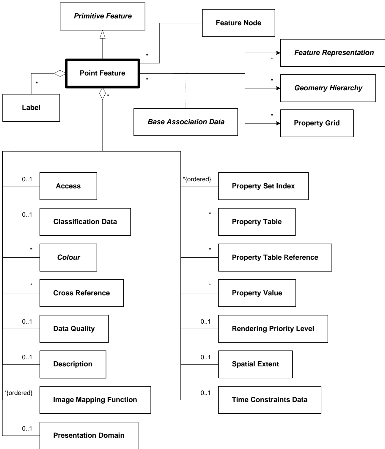
Figure 6.204 — DRM_Point_Feature
