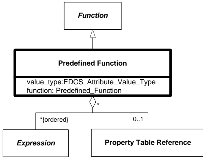
Figure 6.210 — DRM_Predefined_Function
