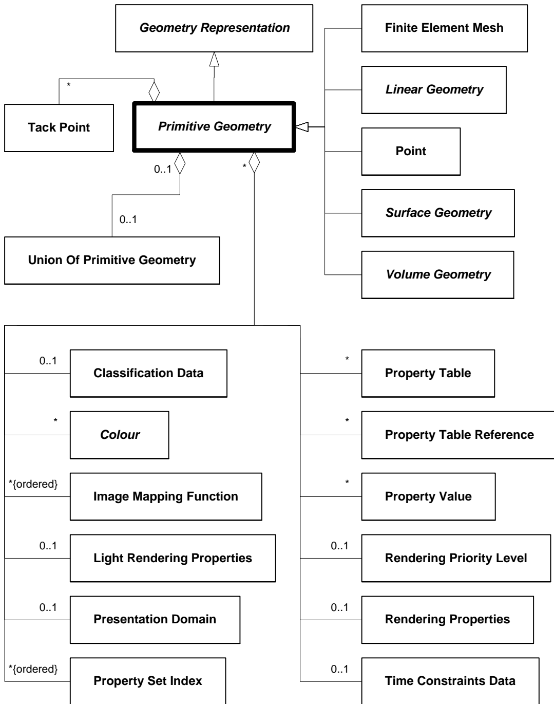
Figure 6.214 — DRM_Primitive_Geometry
