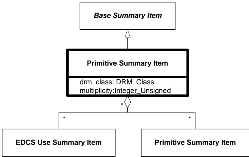
Figure 6.216 — DRM_Primitive_Summary_Item
