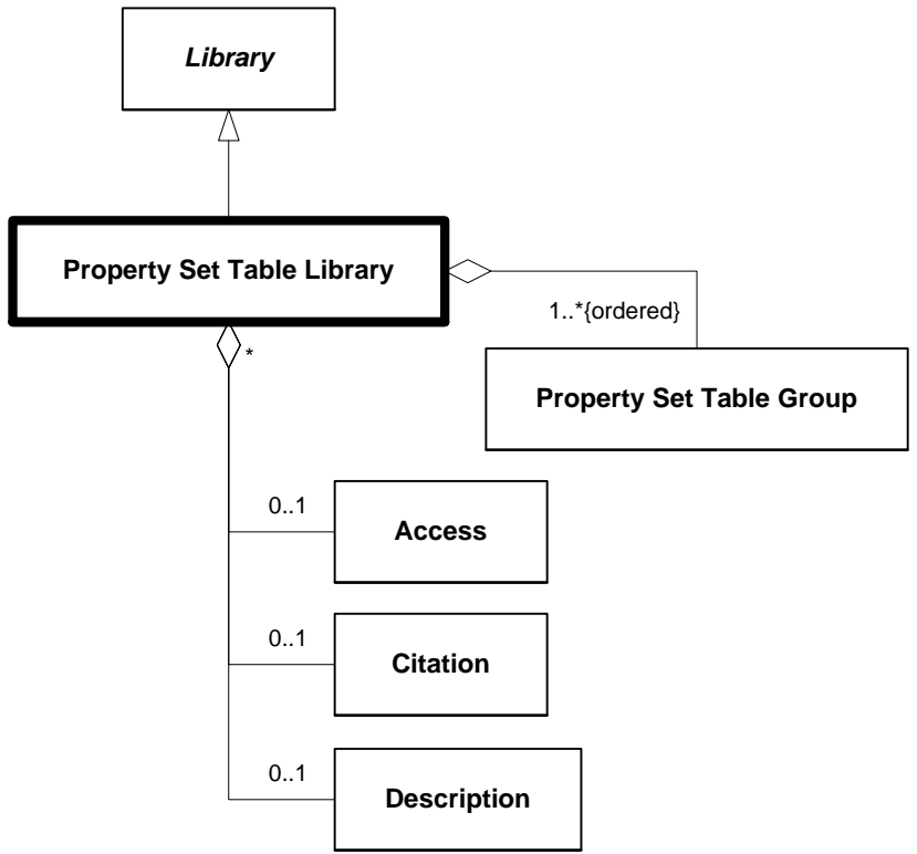
Figure 6.232 — DRM_Property_Set_Table_Library
