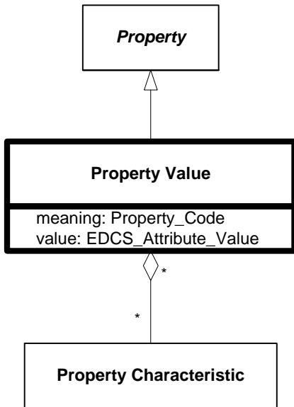
Figure 6.240 — DRM_Property_Value
