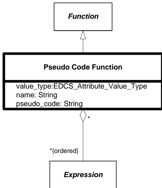
Figure 6.245 — DRM_Pseudo_Code_Function
