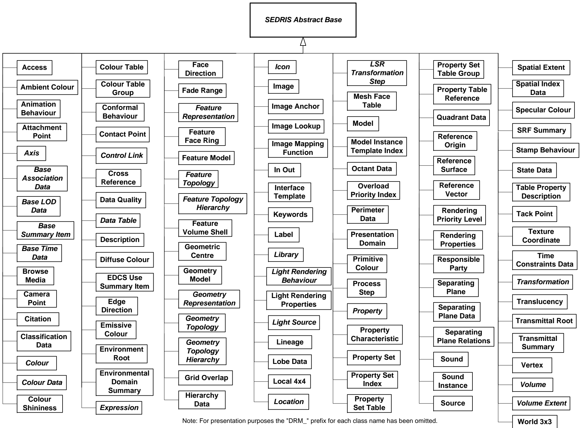
Figure 6.279 — DRM_SEDRIS_Abstract_Base
