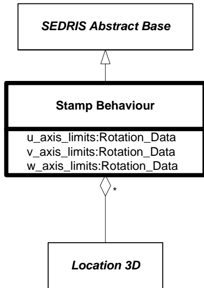
Figure 6.308 — DRM_Stamp_Behaviour
