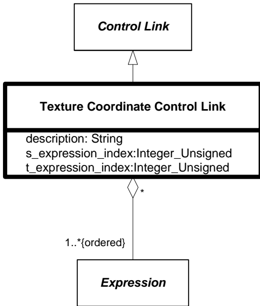
Figure 6.326 — DRM_Texture_Coordinate_Control_Link
