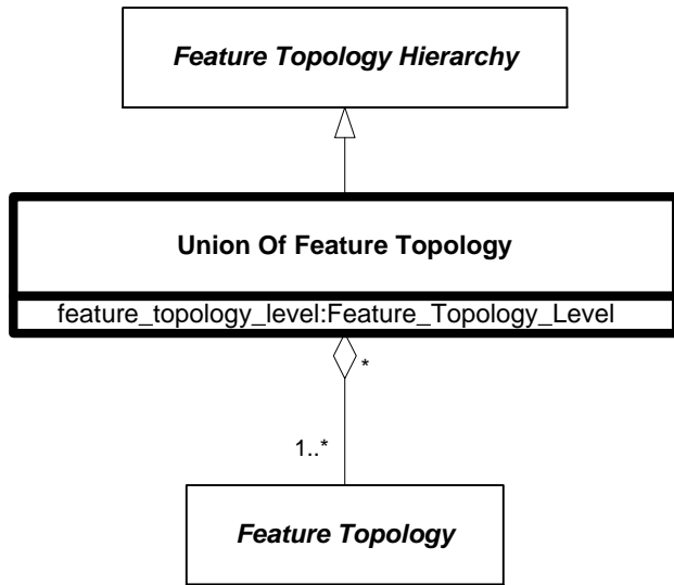
Figure 6.347 — DRM_Union_Of_Feature_Topology
