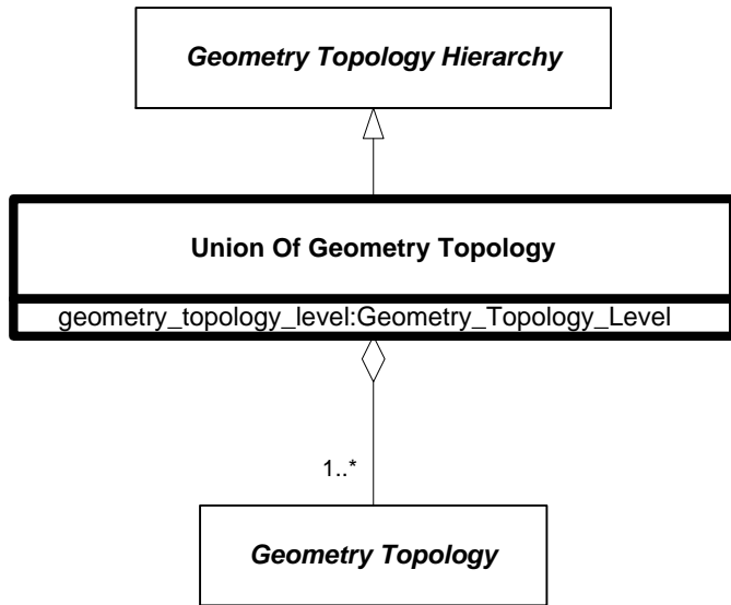
Figure 6.351 — DRM_Union_Of_Geometry_Topology
