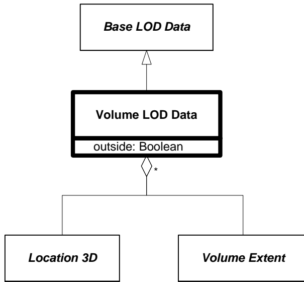
Figure 6.359 — DRM_Volume_LOD_Data
