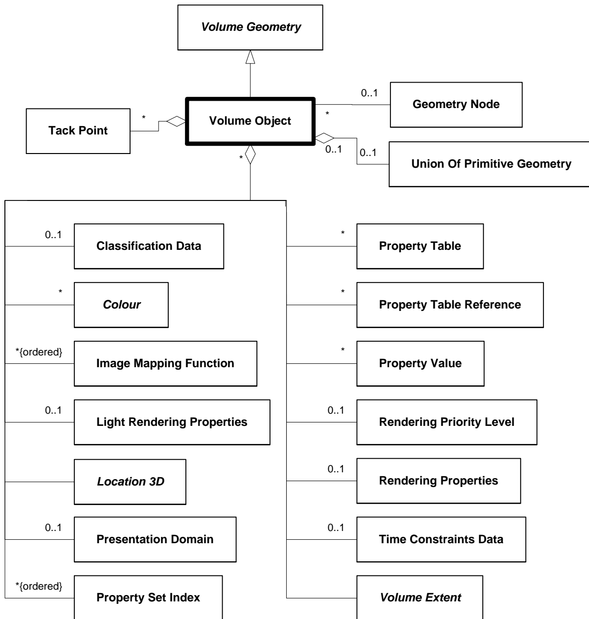
Figure 6.361 — DRM_Volume_Object
