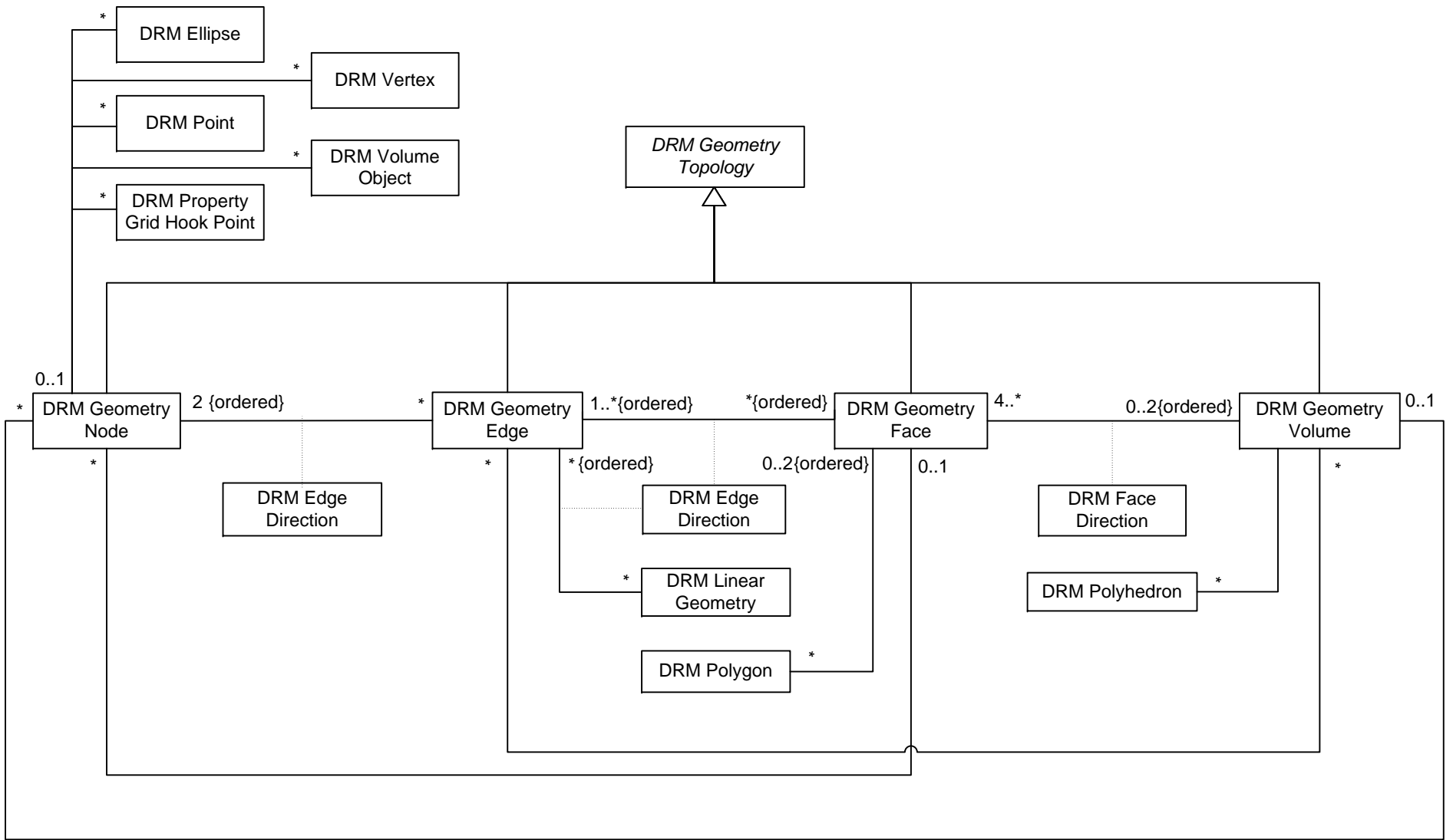
Figure A.11 — Geometry topology
