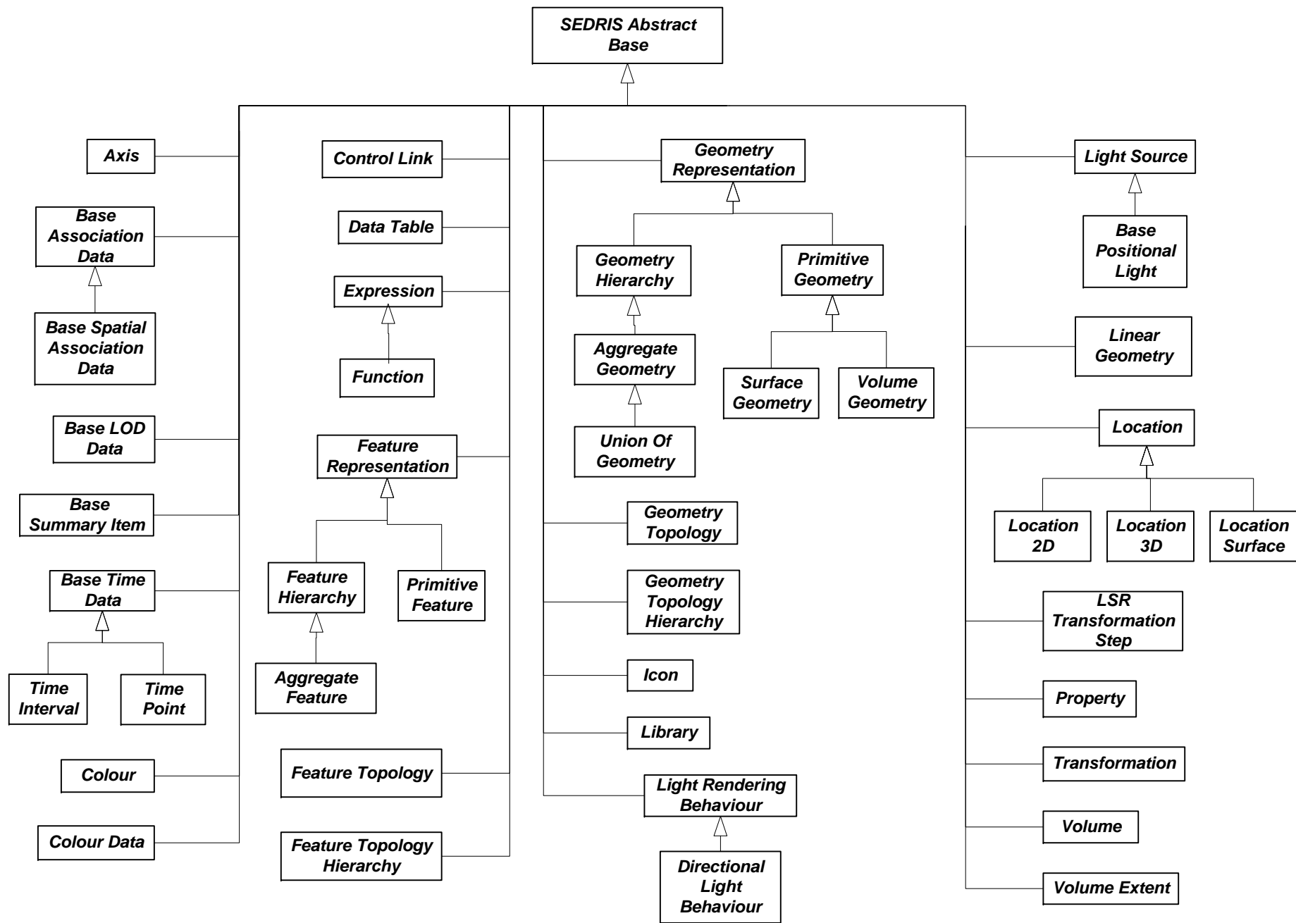
Figure A.24 — Abstract class hierarchy
