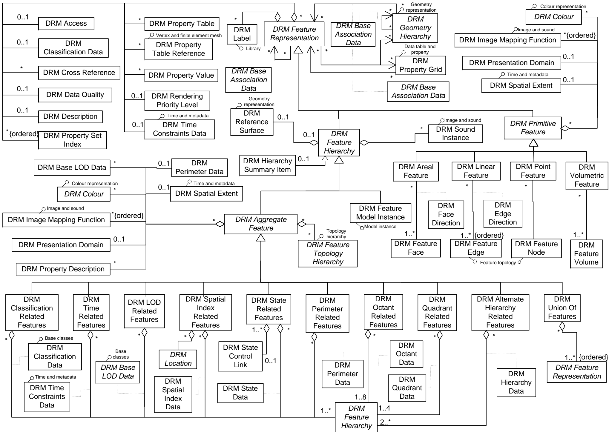
Figure A.9 — Feature representation
